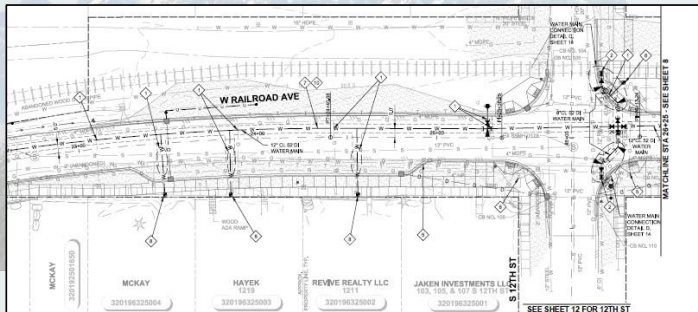
12 th & RAILROAD WATERLINE IMPROVEMENTS
