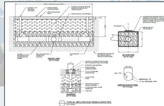
STORM DRAINAGE INFILTRATION TRENCH DETAIL
